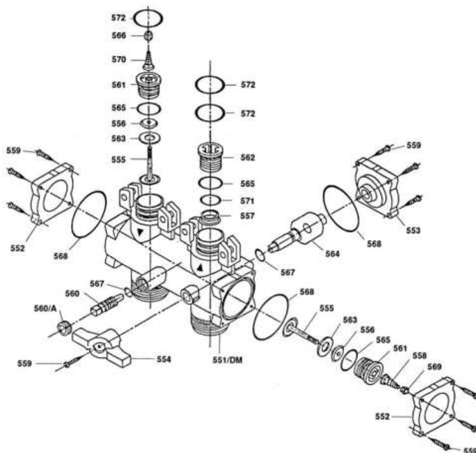
VALVOLA BY-PASS CHIUSA
